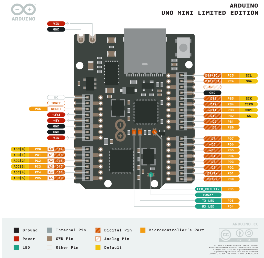
Pinout
